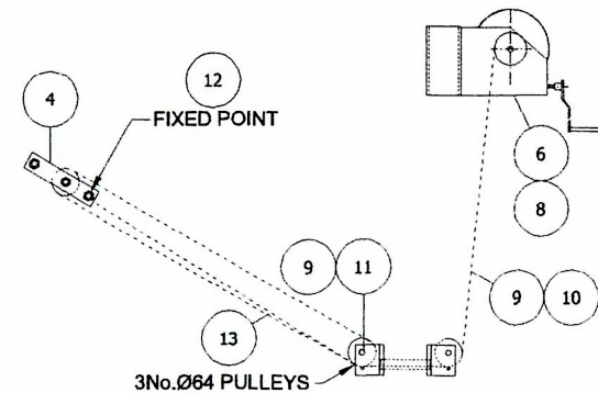
RAISING/LOWERING PULLEY ARRANGEMENT
