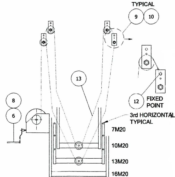
EXTENSION PULLEY ARRANGEMENT
